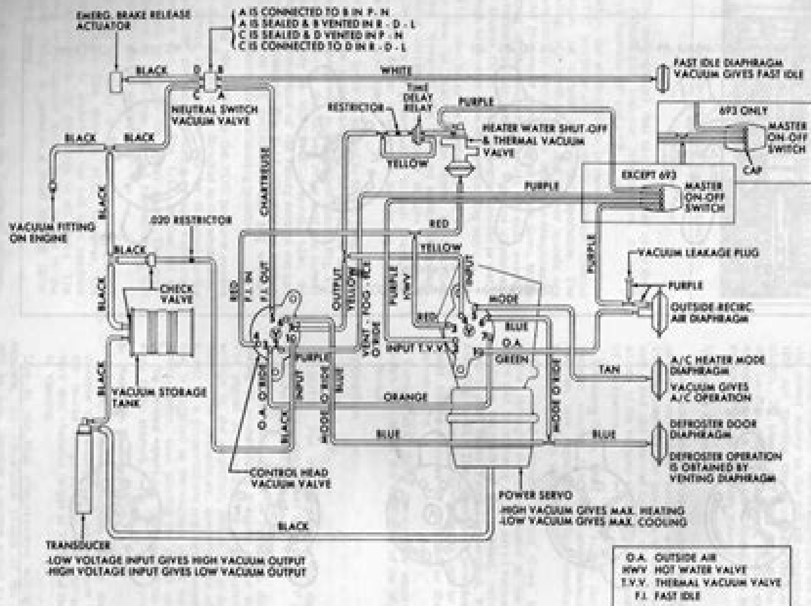
Fig. 1-13 Automatic Climate Control Vacuum Schematic
