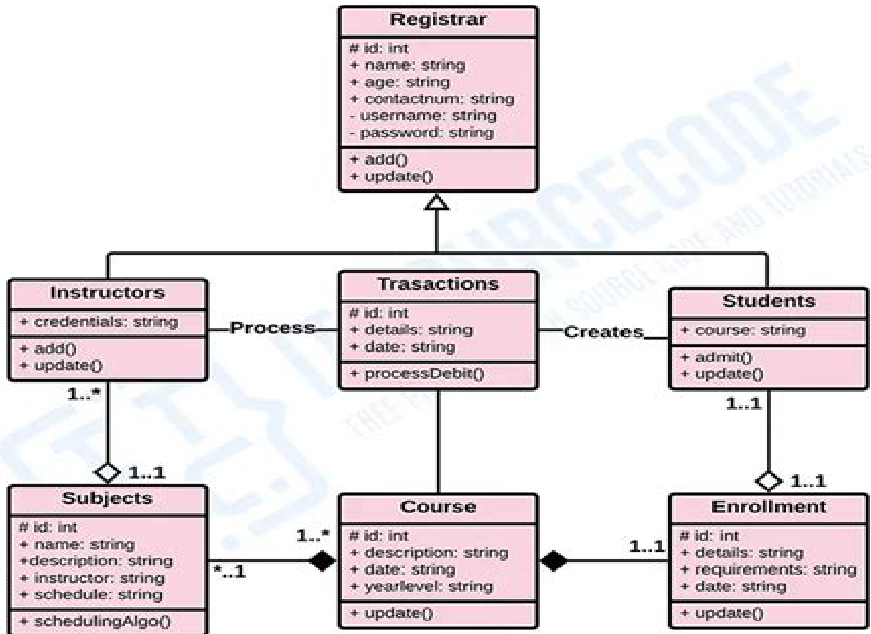
CLASS DIAGRAM
