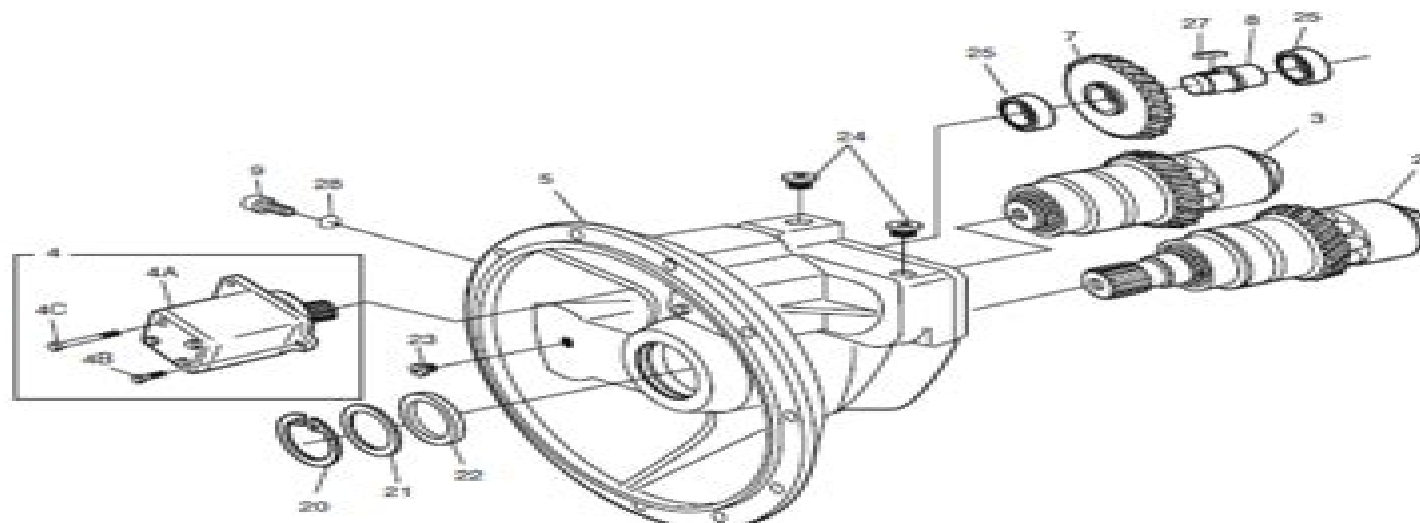
Fig. 4110 MAIN PUMP-PUMP POMPE
