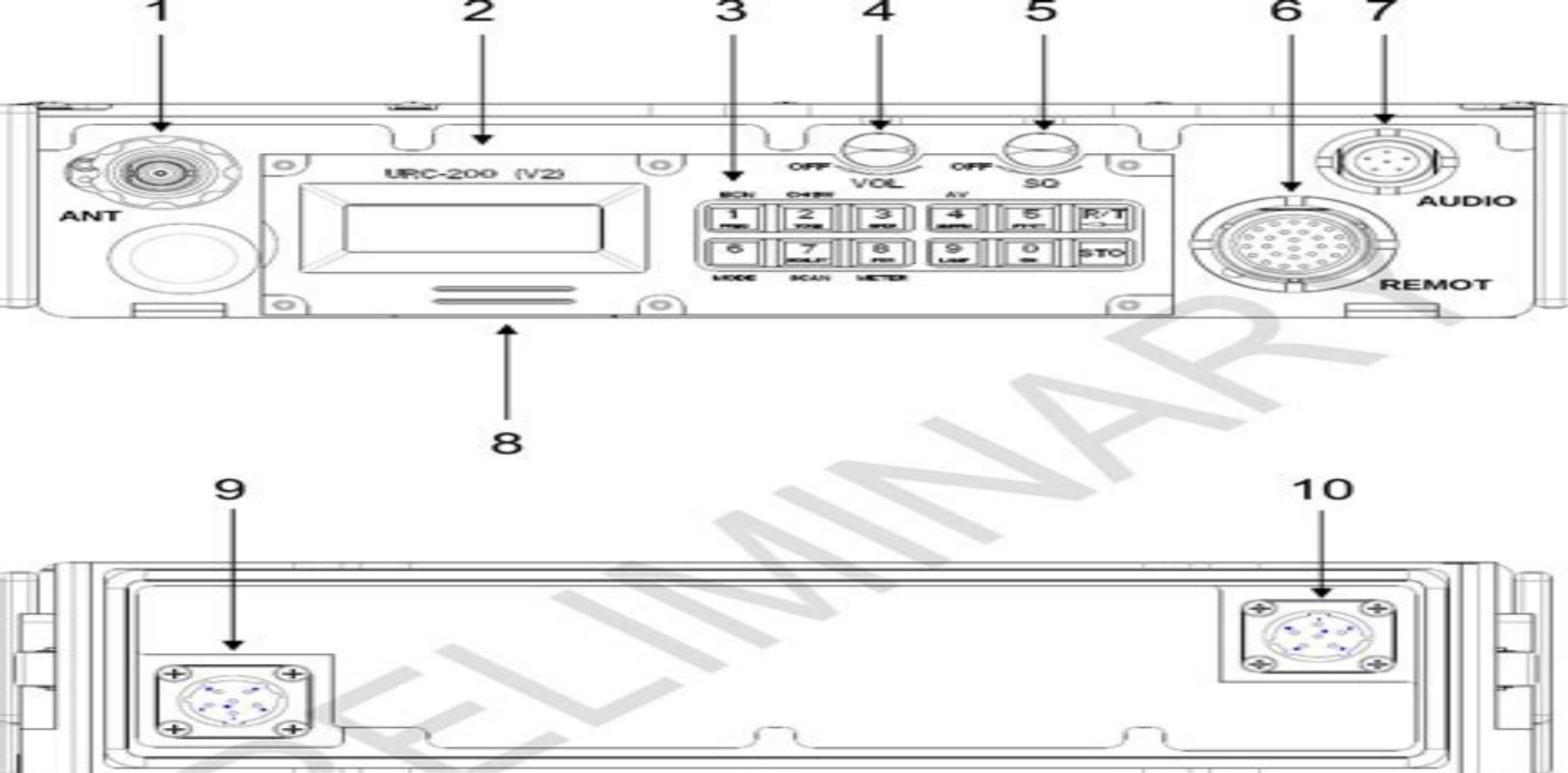
Figure 2-1. URC-200 (V2) Front and Rear Panel Controls, Indicators and Connectors
