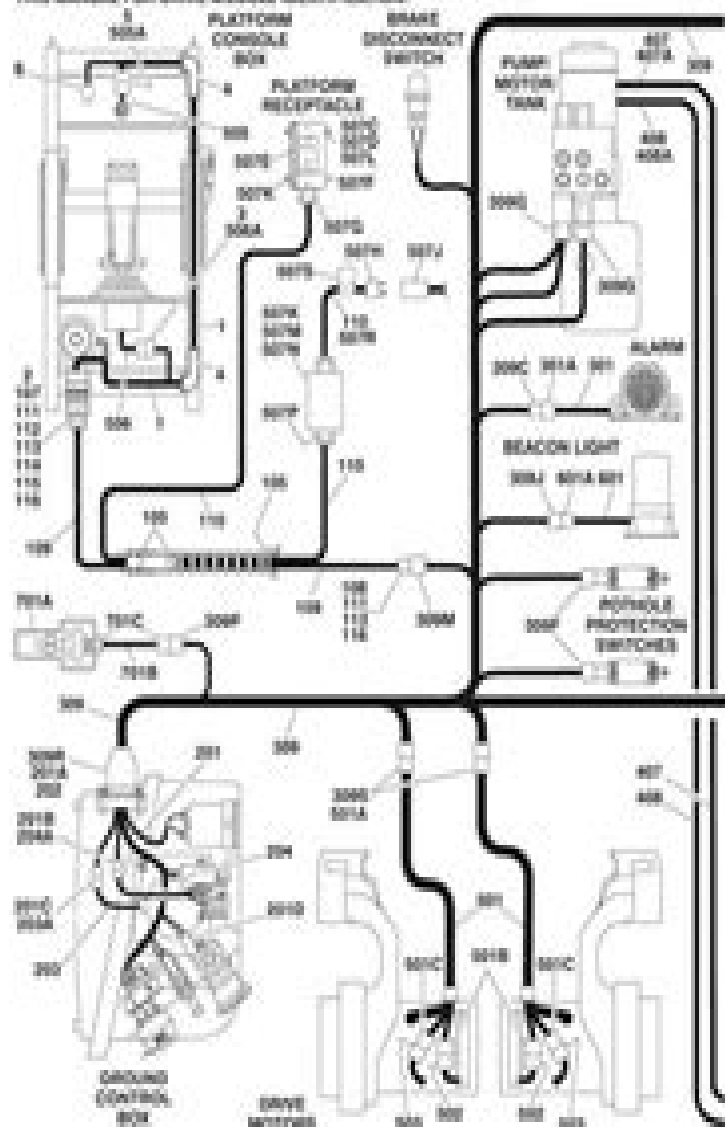
FIGURE 7-4. ELECTRICAL CONNECTORS INSTALLATION (MACHINES WITH 16010004M DRIVE MODULE)
