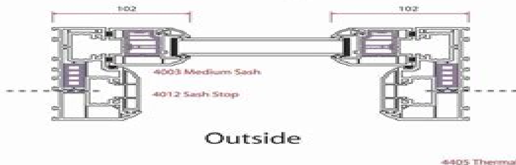
Horizontal section through bottom sash
