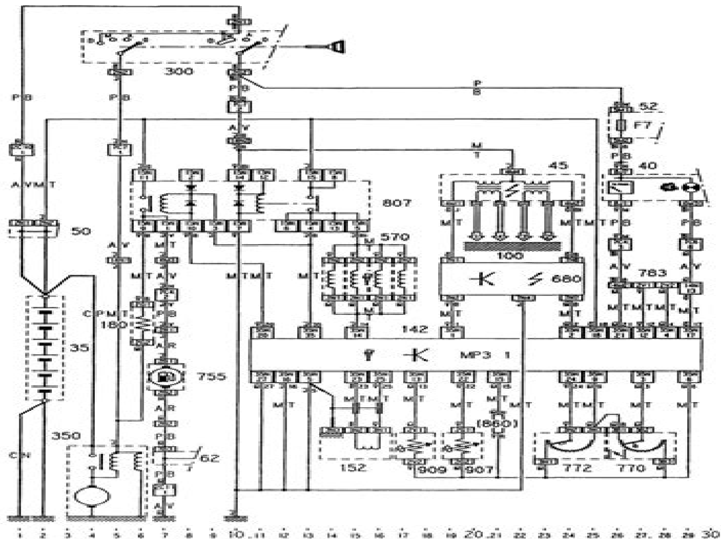
Engine electrical systems - 1905 cc non-catalyst (D6E/XU9JA K)
