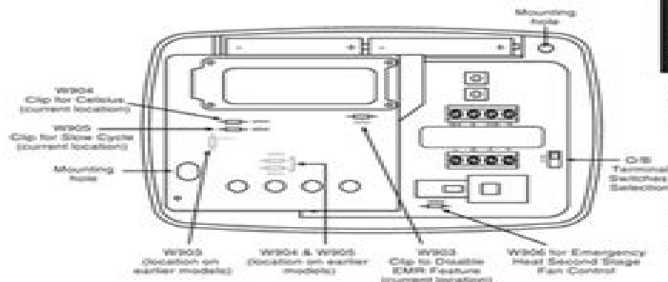
Figure 1. Thermostat base
