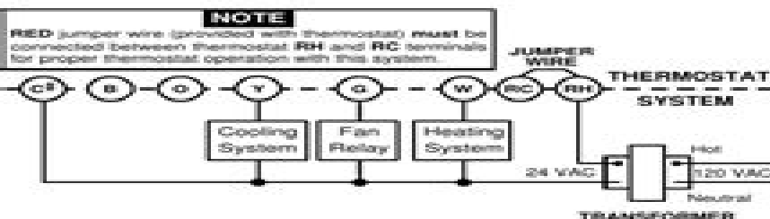
Figure 4. Typical wiring diagram for heat/cool, 4-wire, single transformer systems
