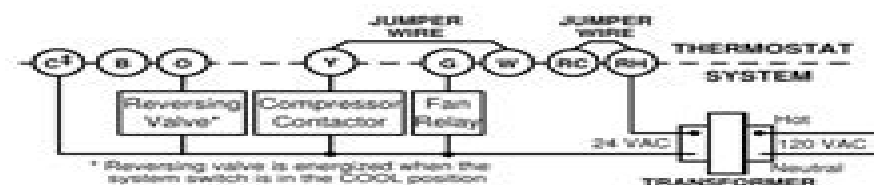
Figure 6. Typical wiring diagram for heat pump with reversing valve energized in COOL
