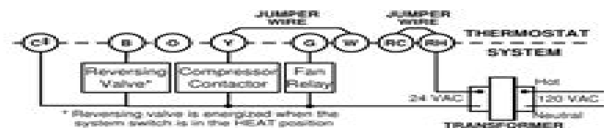
Figure 7. Typical wiring diagram for heat pump with reversing valve energized in HEAT
