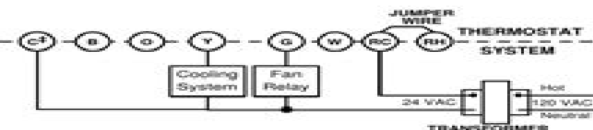
Figure 3. Typical wiring diagram for cool only, 3-wire, single transformer systems
