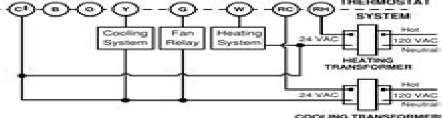
Figure 5. Typical wiring diagram for heat/cool, 5-wire, two-transformer systems
