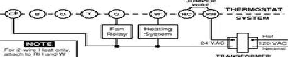
Figure 2. Typical wiring diagram for heat only, 3-wire, single transformer systems
