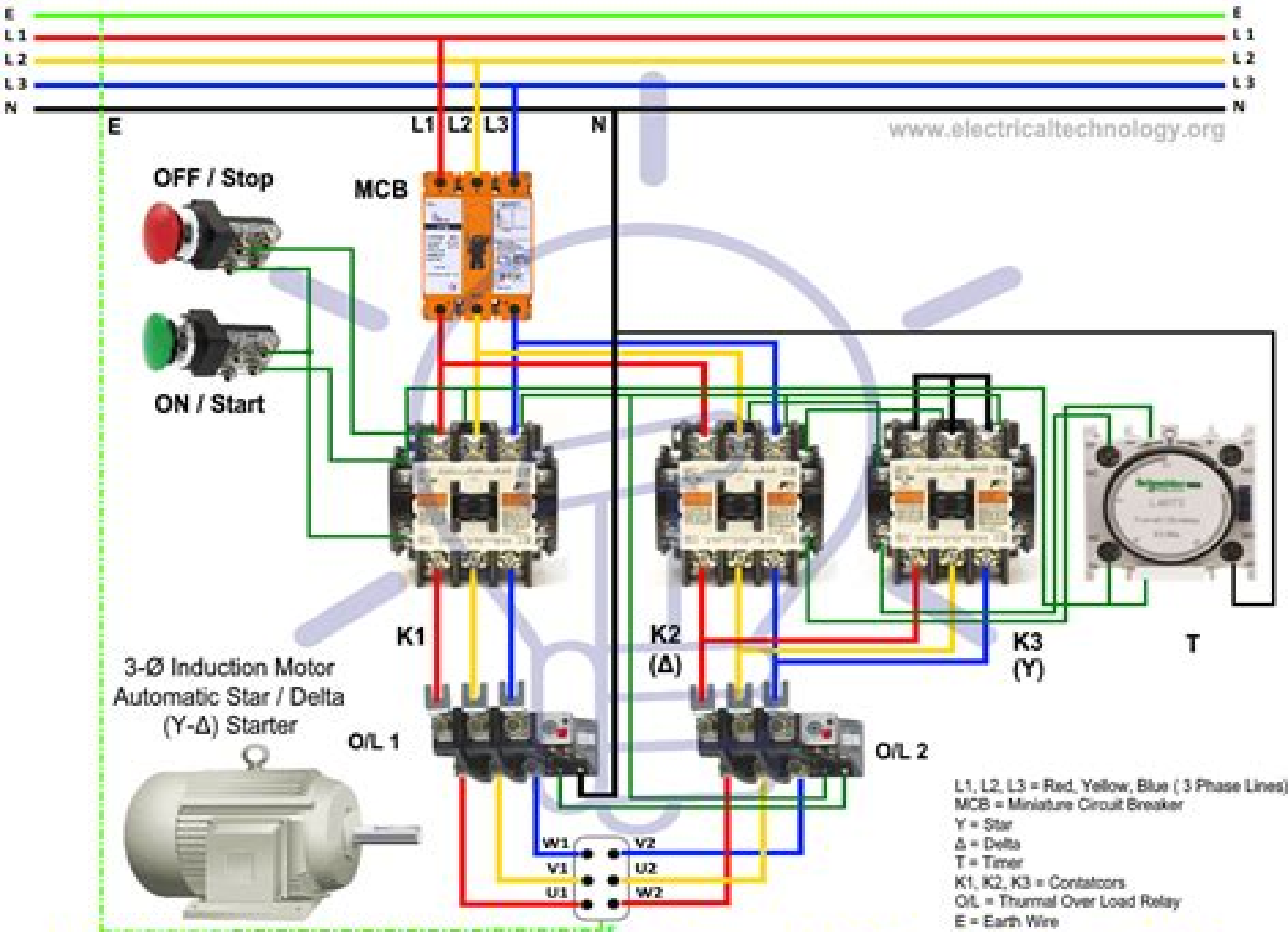
Automatic Star / Delta (Y-Δ) Starter with Timer for 3-Phase Induction Motor
