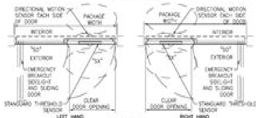
LEFT HAND PLAN VIEW RIGHT HAND
