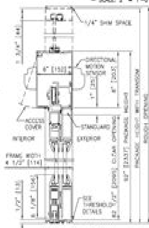
VERTICAL SECTION
