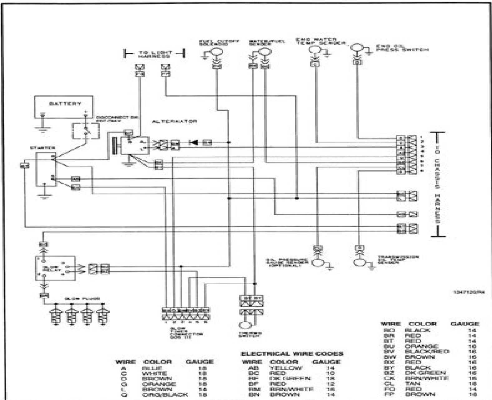
FIGURE 6. WIRING SCHEMATIC FOR THE ISUZU DIESEL ENGINE
