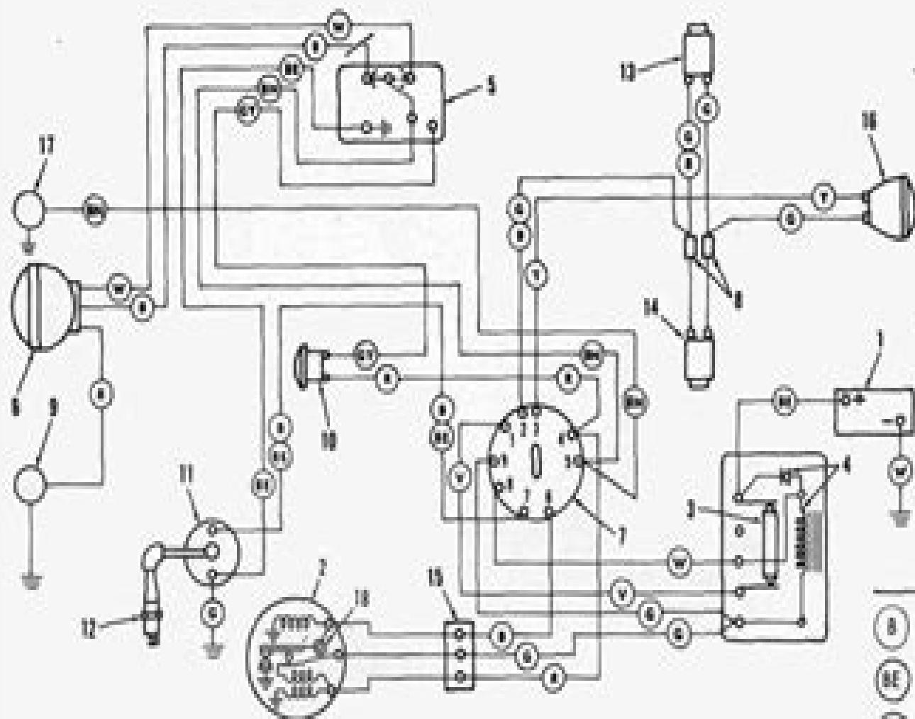
1972 M125 (Rapido) Wiring Diagram
