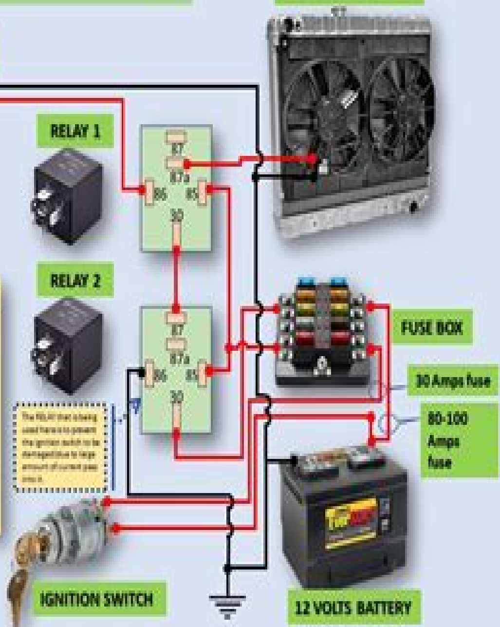
RADIATOR WITH FAN
