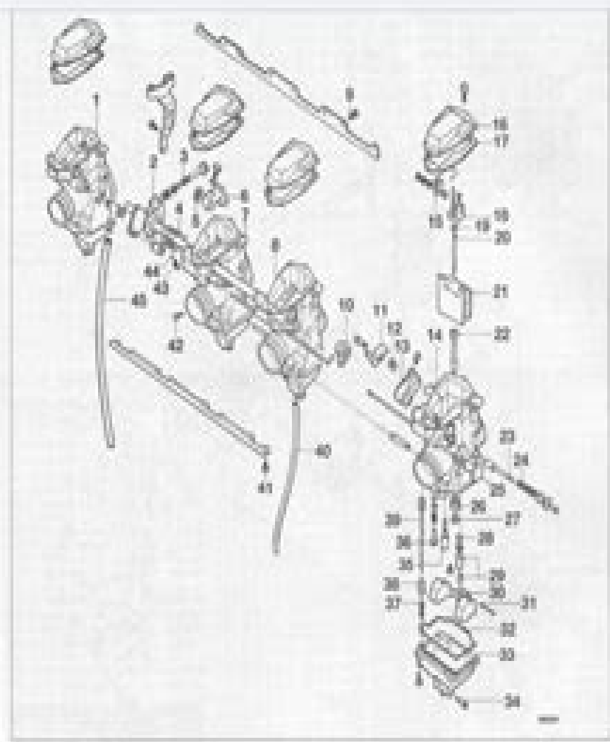
61 W2000 carburetor - exploded view
