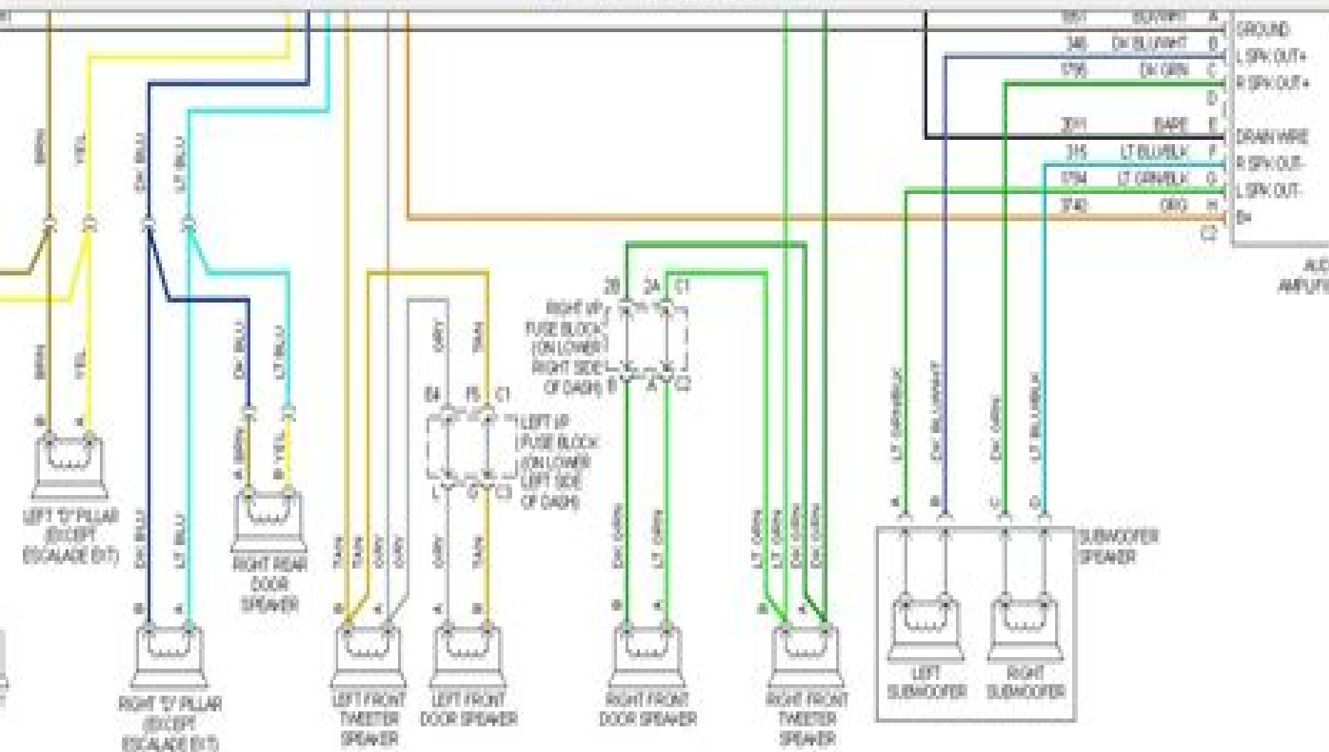
Fig. 14 Multi-Line Radio Circuit, W/ Rear Seat Audio (2 of 3)
