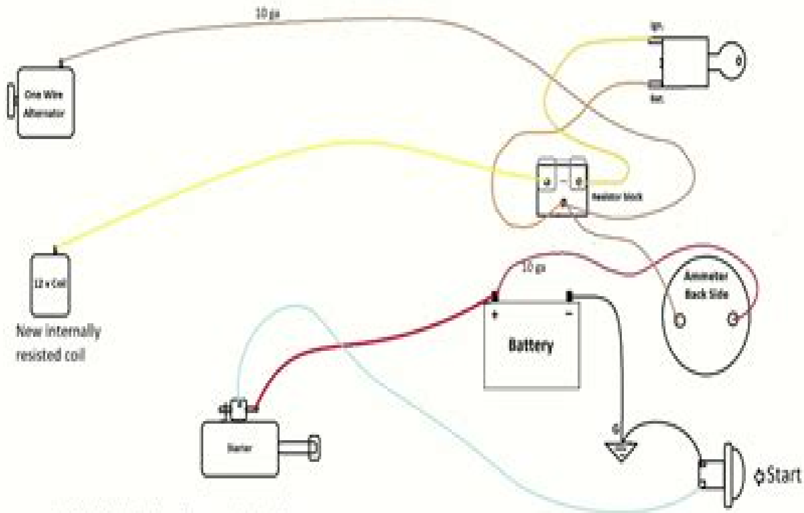
Ford 9N / 2N Wiring diagram. Using 12 v system.
