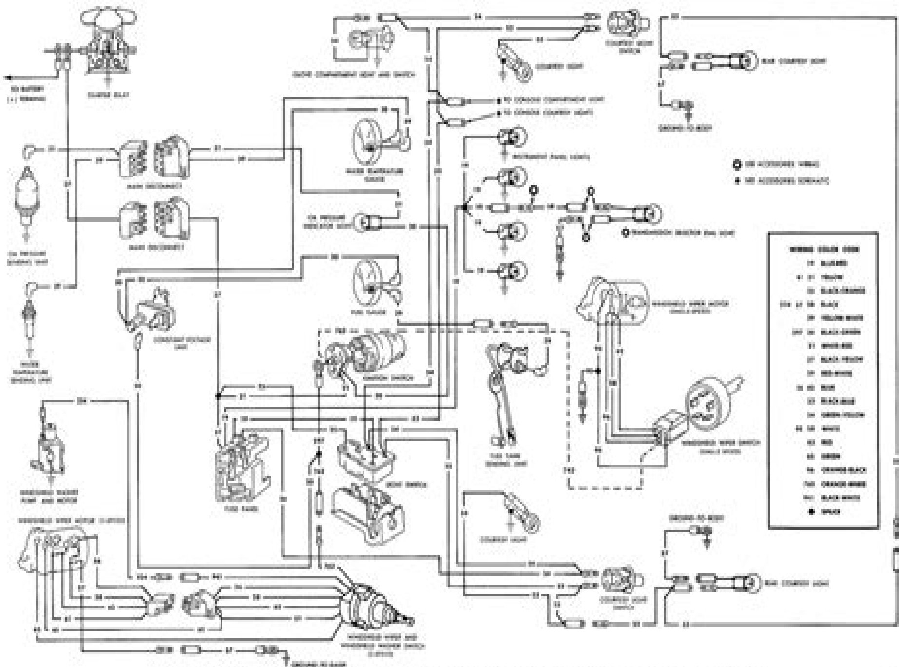
1965 MUSTANG INTERIOR LIGHTING, WINDSHIELD WIPERS AND GAUGES
