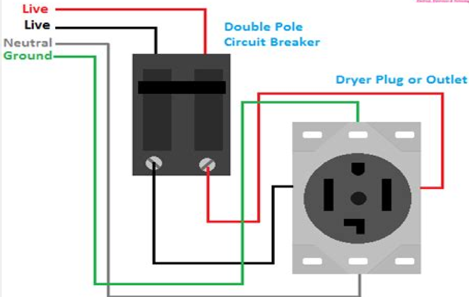
4 Prong Dryer Outlet Wiring Diagram
