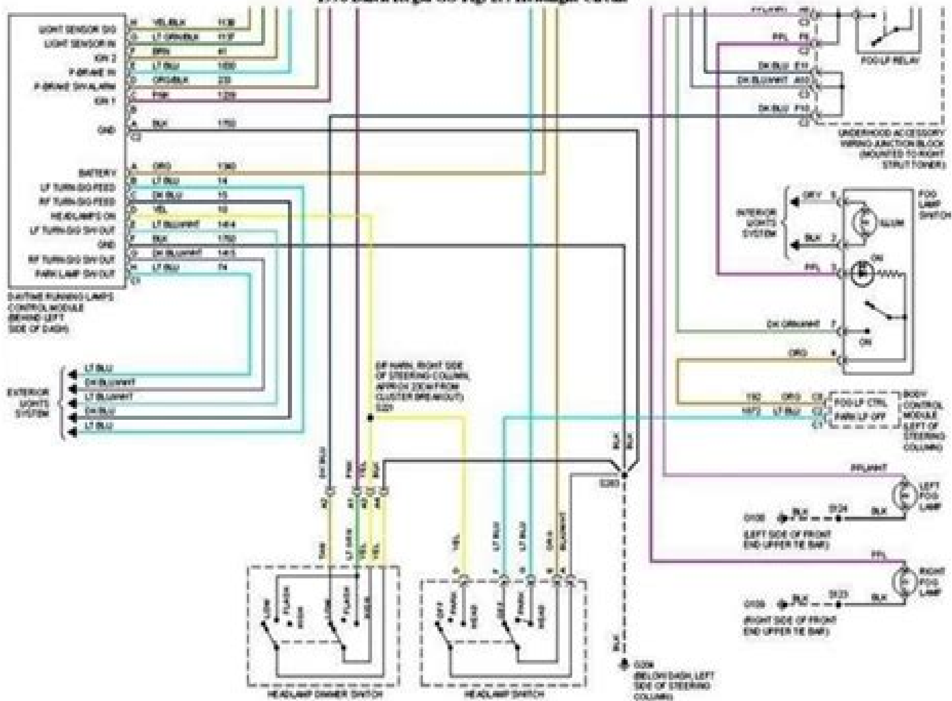
1993 Buick Regal GS-Fig. 25: Headlight Circuit
