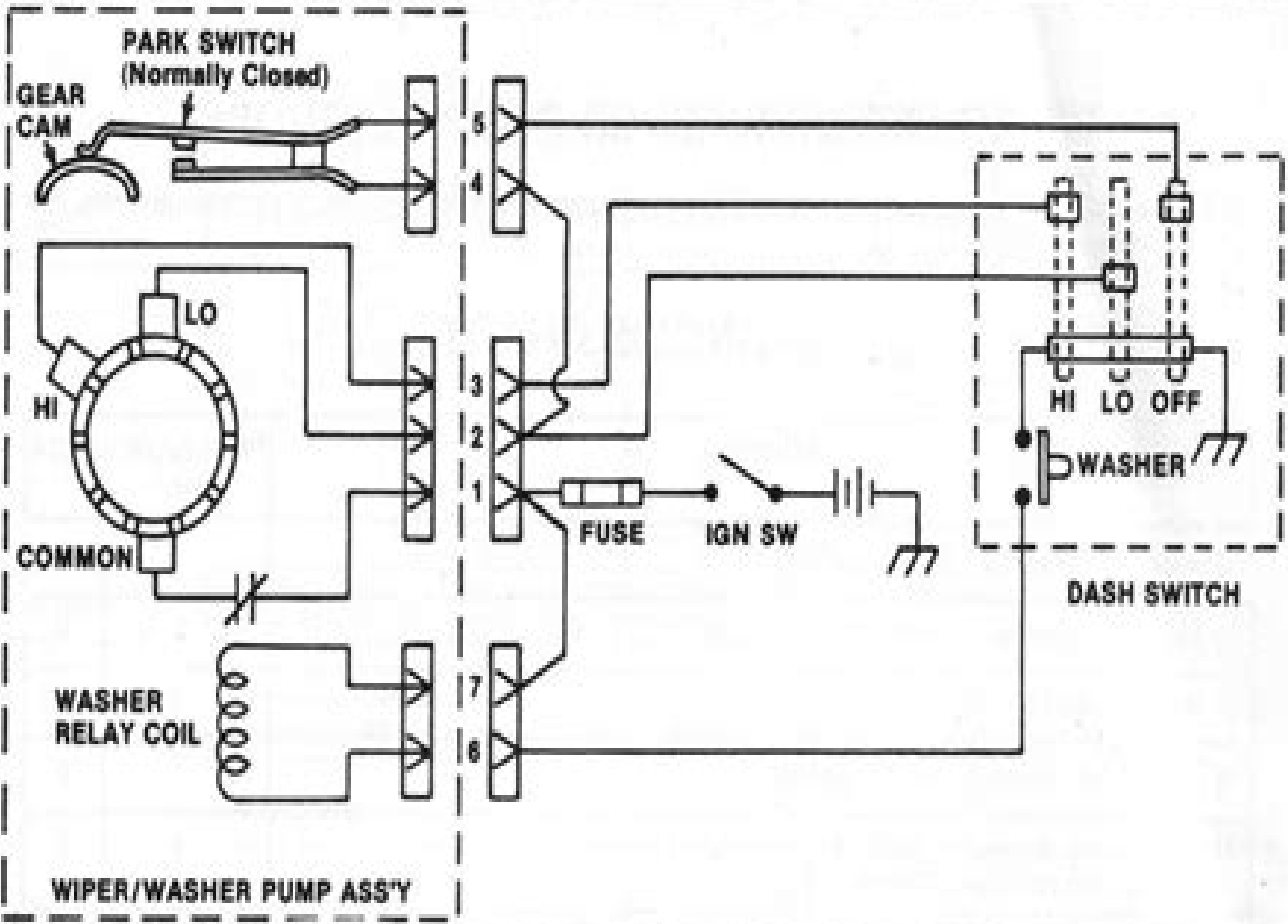
Fig. 8-4-Wiper Motor Schematic
