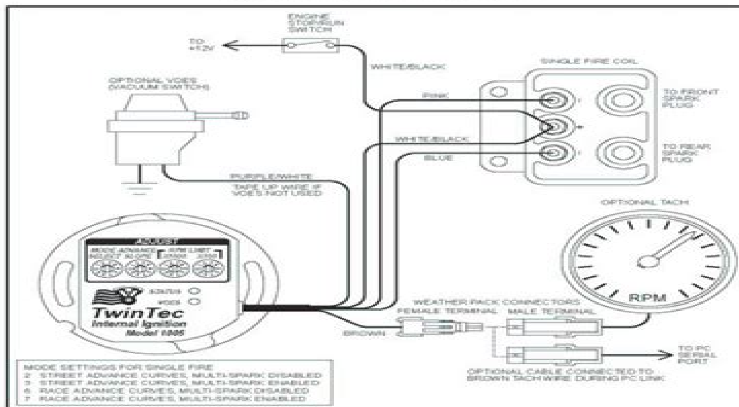
Figure 5 - Single Fire Wiring Diagram
