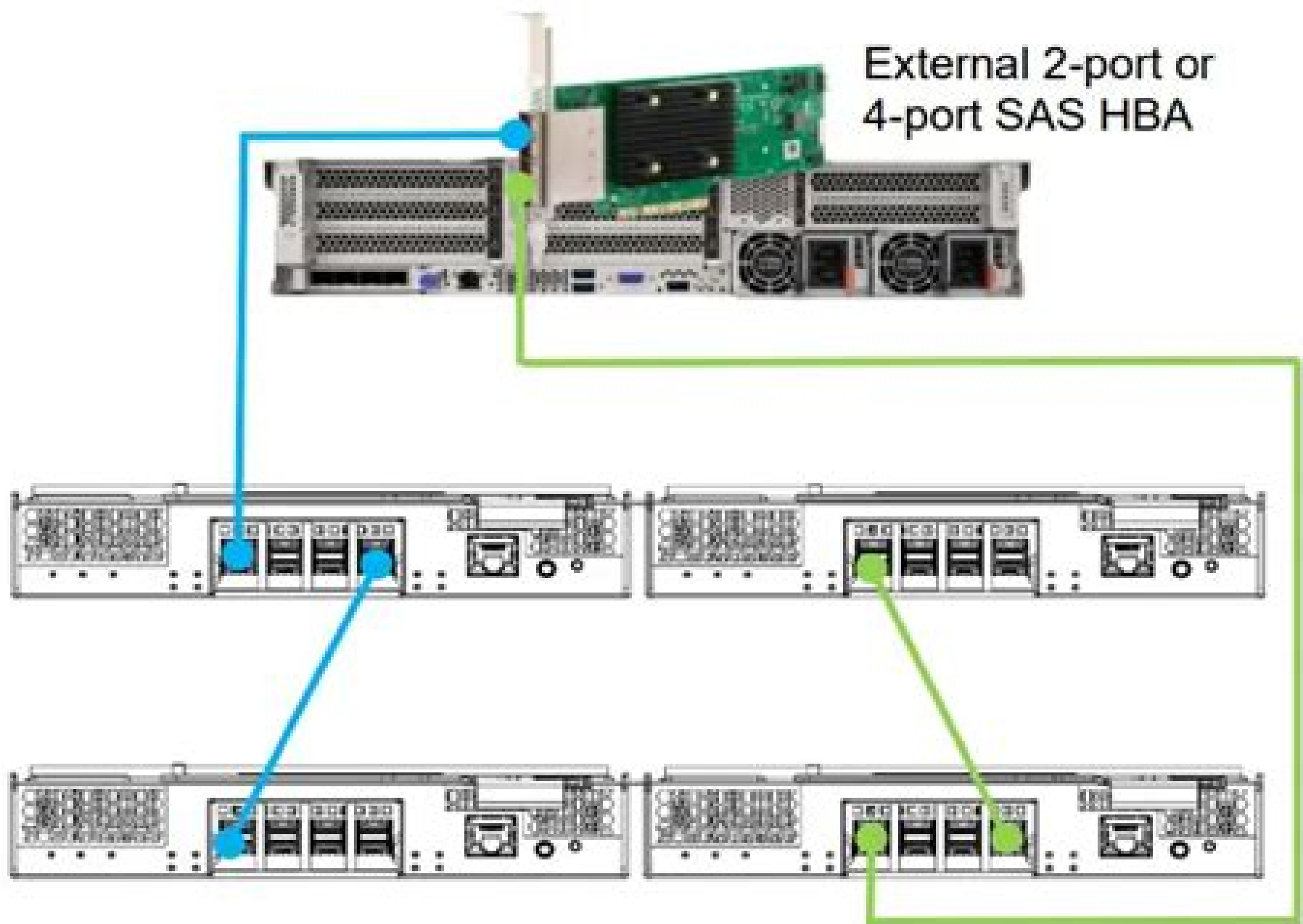
Figure 8: Single SAS HBA for up to two enclosures
