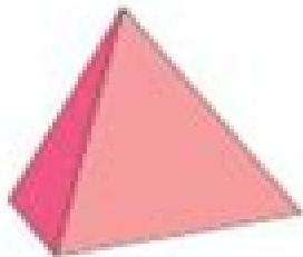
Tetrahedron
