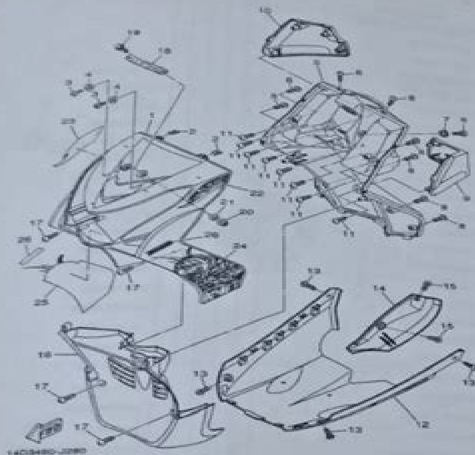
FIG. 28 LEG SHIELD
