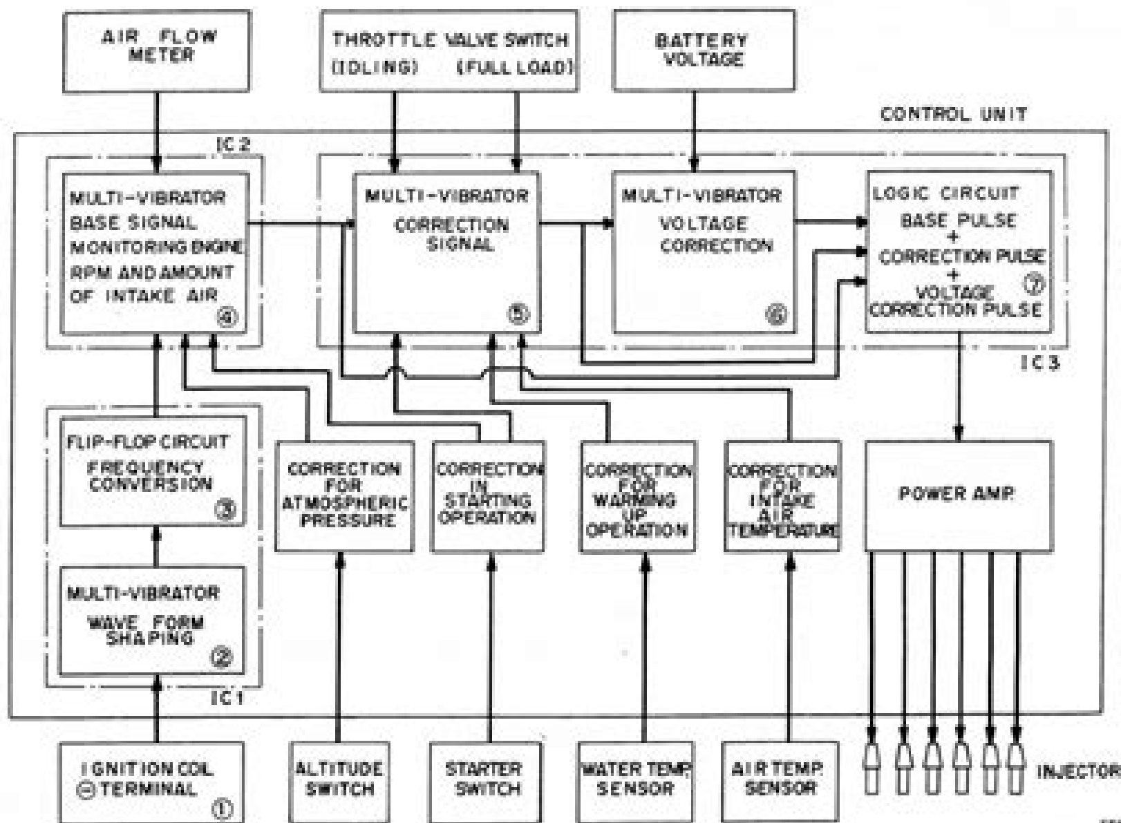
Fig. 17-4 Control unit block diagram
