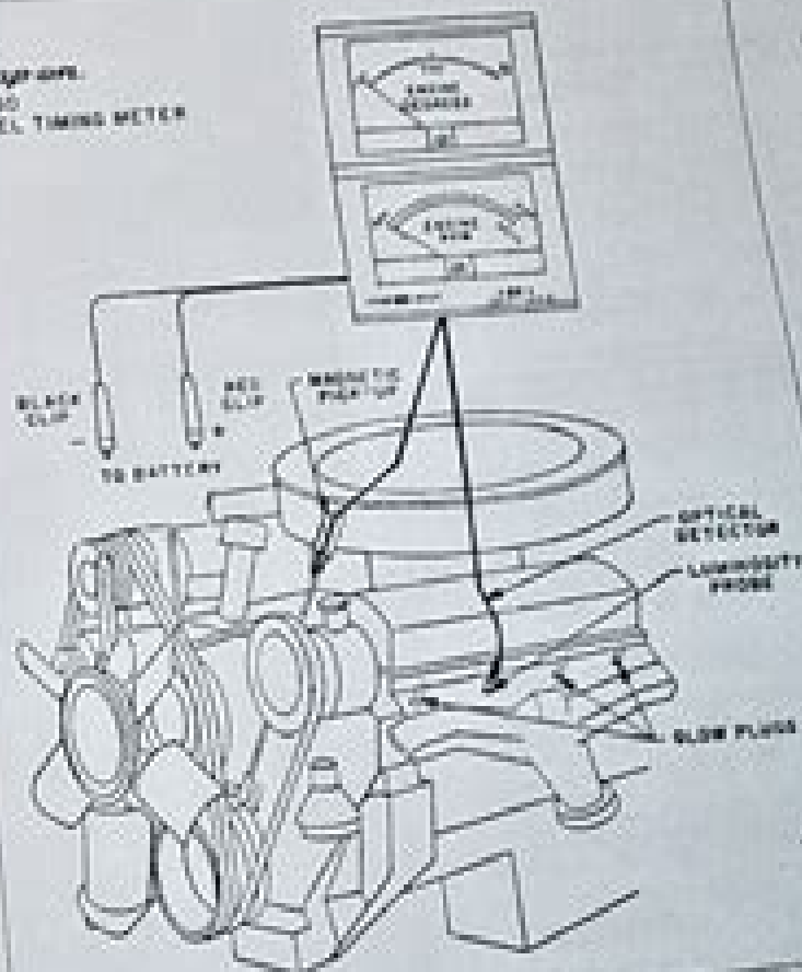
Figure 1 - Typical meter for a 1.6 with 9.5" offset probe holder
