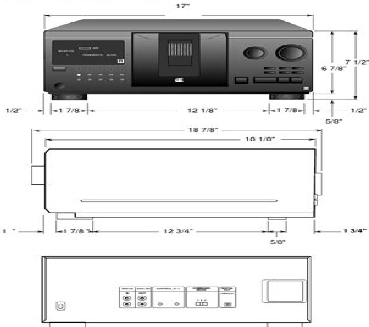
FRONT VIEW
