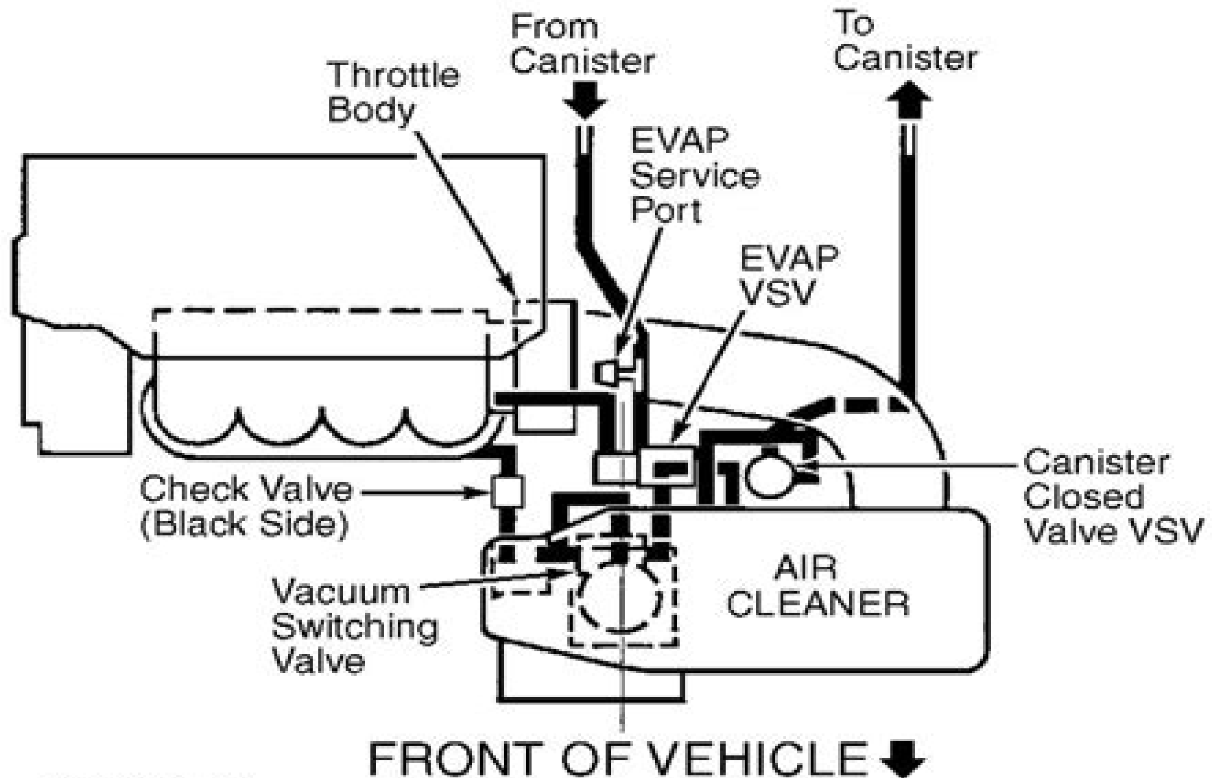
Fig. 14: Vacuum Diagram (Celica 1.8L 4-Cyl. 2ZZ-GE - 2 Of 4) Courtesy of TOYOTA MOTOR SALES, U.S.A., INC.
