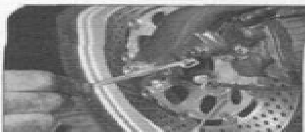
16.5a Some models are equipped with a fork drain screw at the bottom of each fork leg; it can be at the rear, as on this 750 Katana (GSX750F)...
