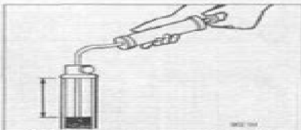
16.9 Measure oil level in the fork; this measuring tool can be easily fabricated, but a tape measure will also work; add or drain oil to correct the level
