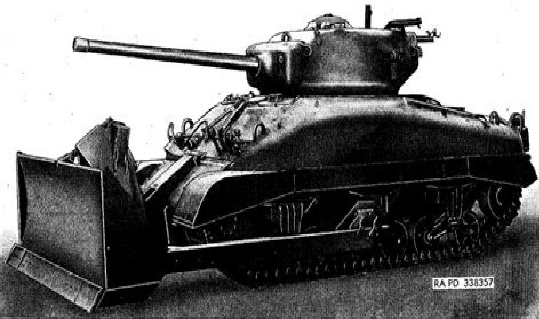
Figure 1. Bulldozer M1 mounted on medium tank M4A1 (standard vertical suspension)—left side.
