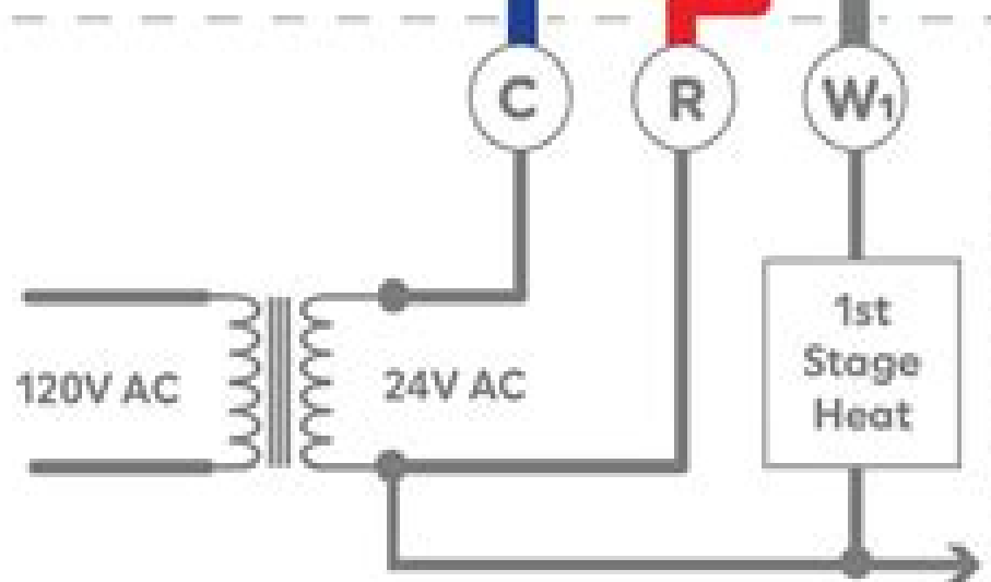
Furnace Connections
