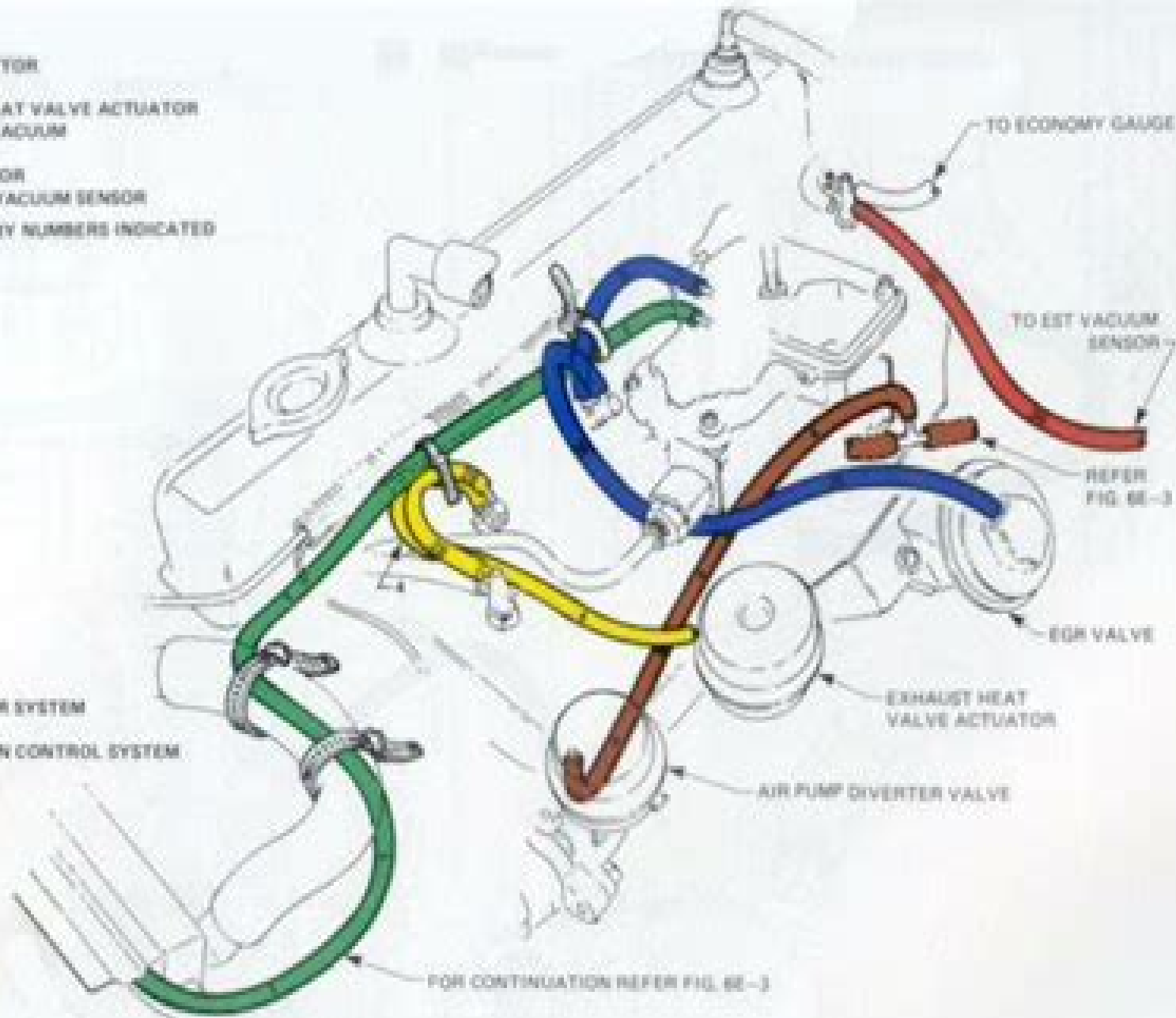
EMISSION HOSE ROUTING – EST ENGINES WITH AUTOMATIC TRANSMISSION
