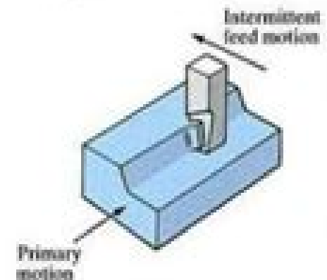
Production of a flat surface
