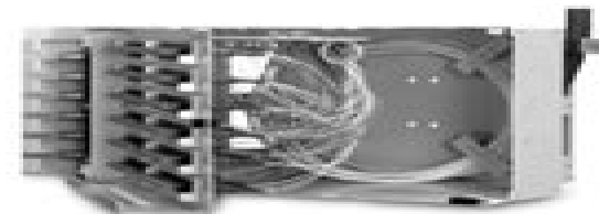
Swing-out Bulkhead (Allows Full Access)
