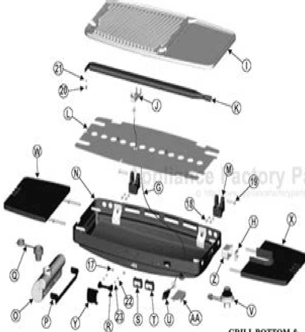
GRILL BOTTOM & BURNER SYSTEM
