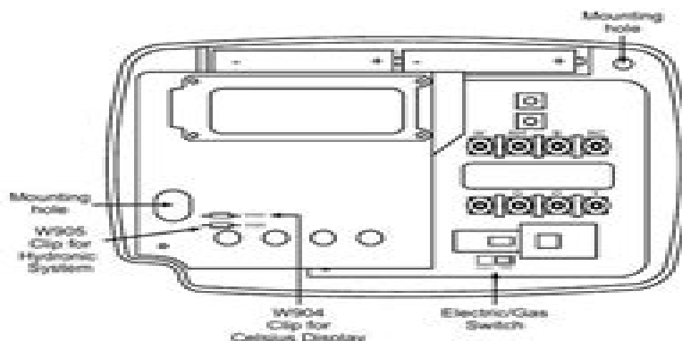
Figure 1. Thermostat base
