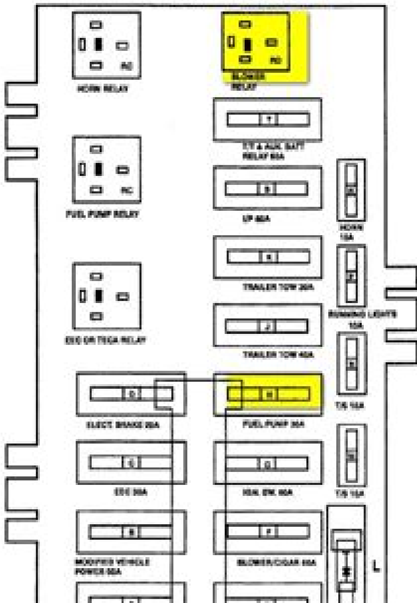
ENGINE COMPARTMENT FUSE PANEL
