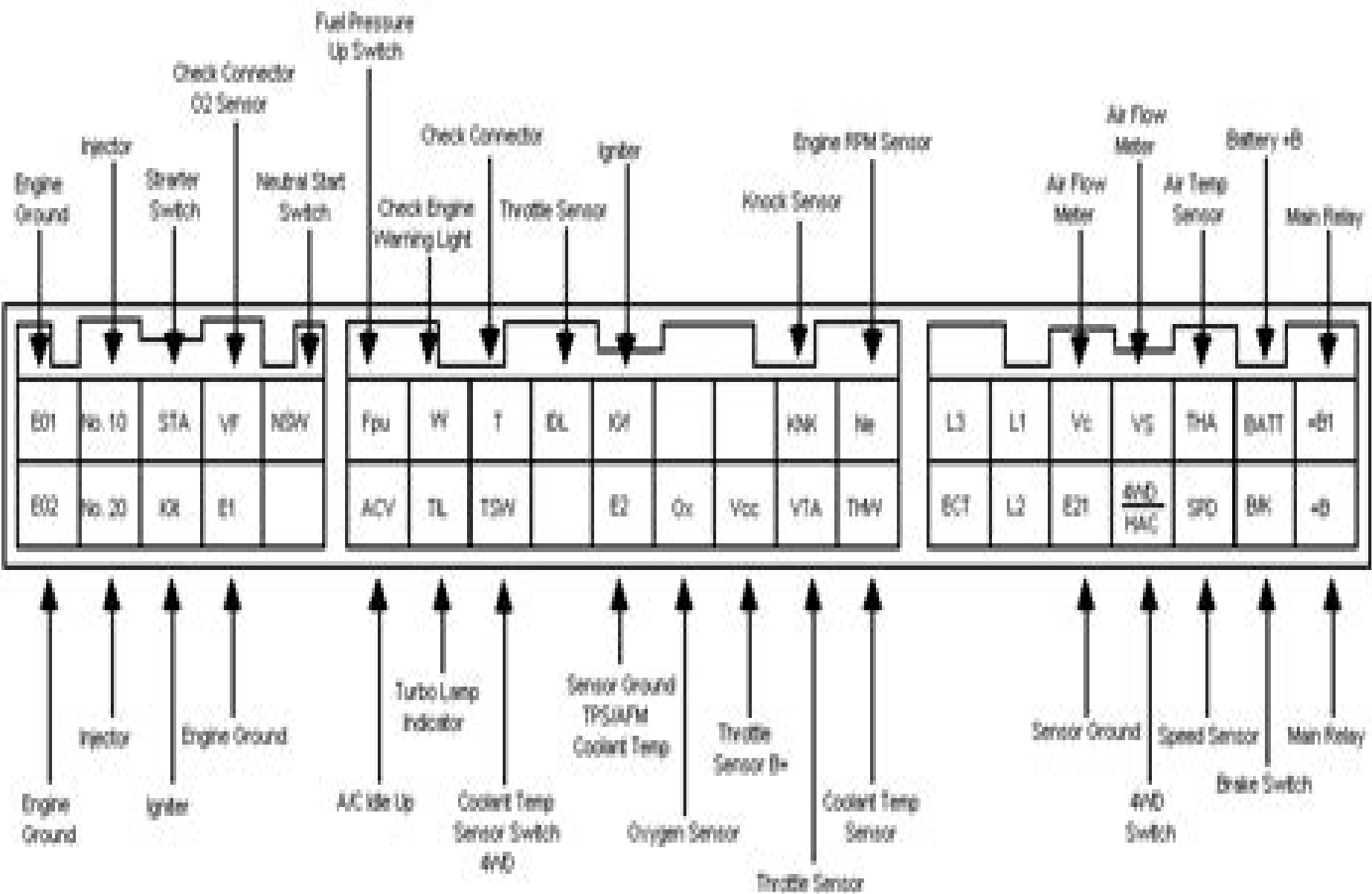
ECU Pinouts for 86 Toyota Truck w/23RTE
