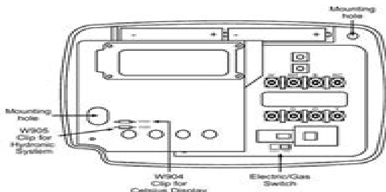
Figure 1. Thermostat base
