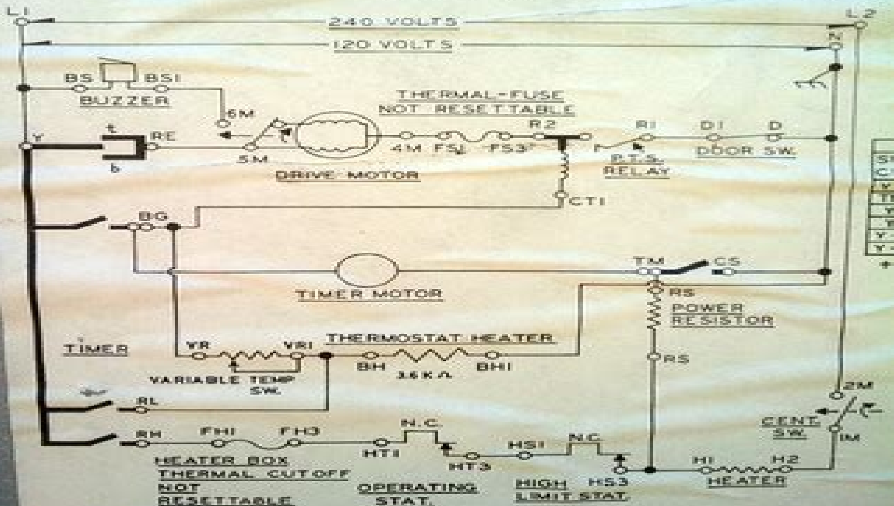
ELECTRIC DRYER WIRING DIAGRAM
