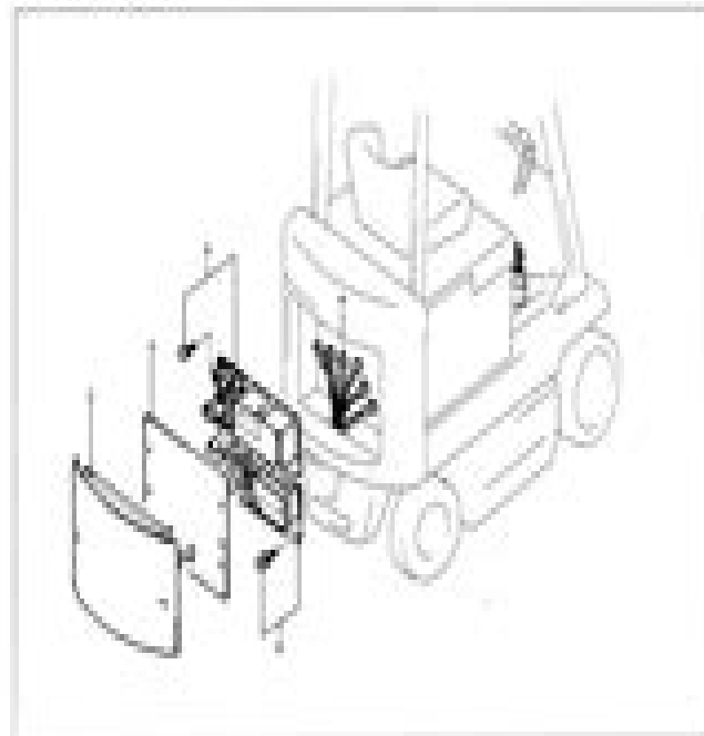
Control Panel ASST - Removal Procedure
