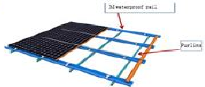
Installation node diagram of M rail with beam:
