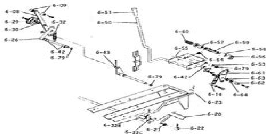
Plate 6.5 BRAKE, SPEED CONTROL LINKAGE
