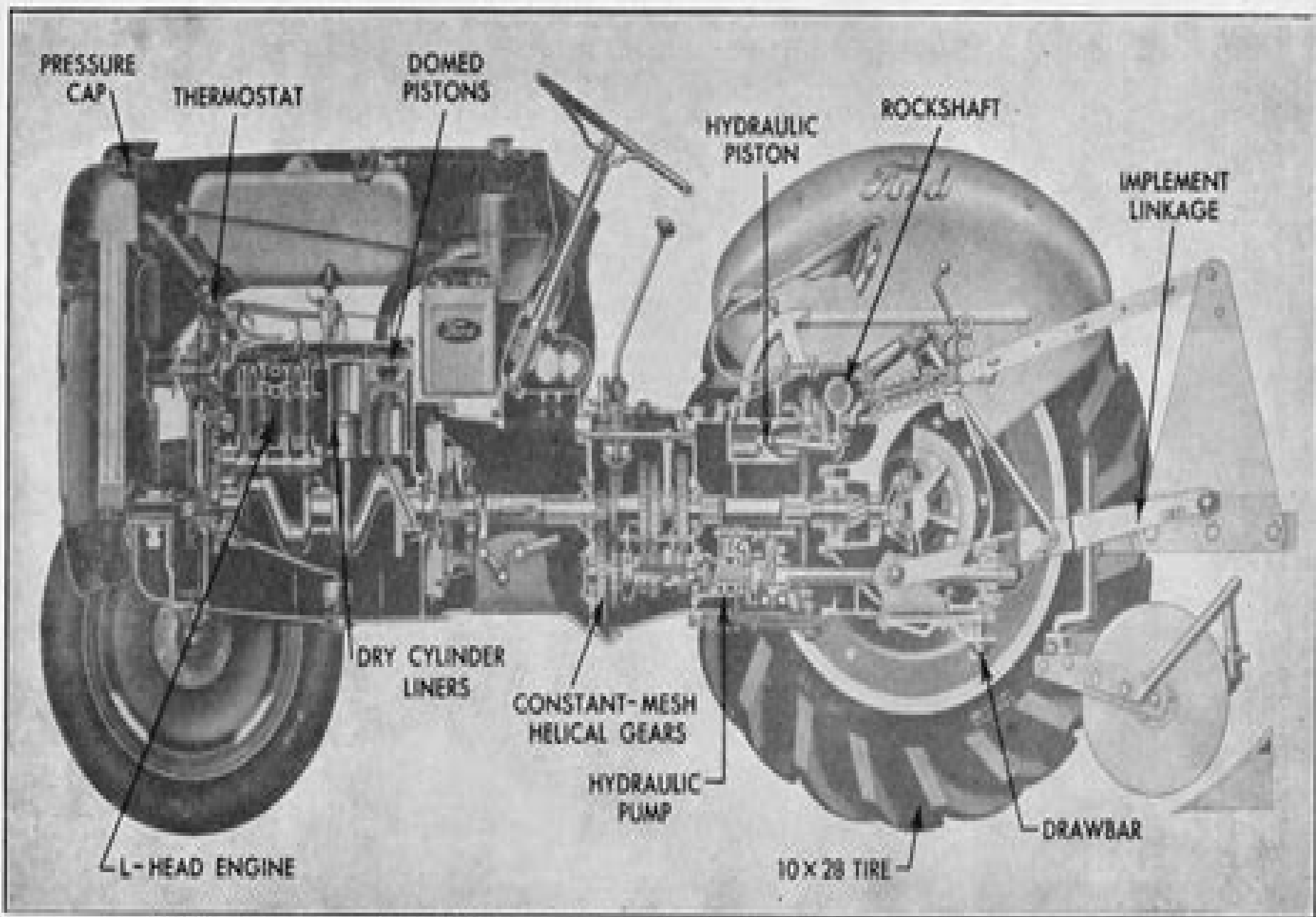
FIG. 271. Sectional view of the Ford 8N tractor showing the features of the tractor which is discussed in the text.
