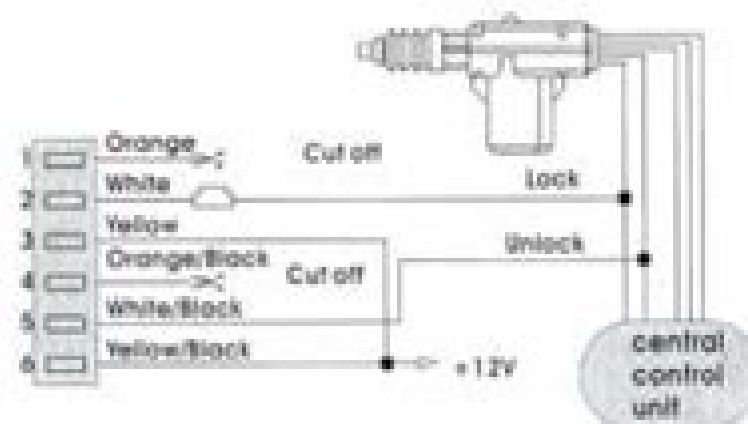
Positive trigger
