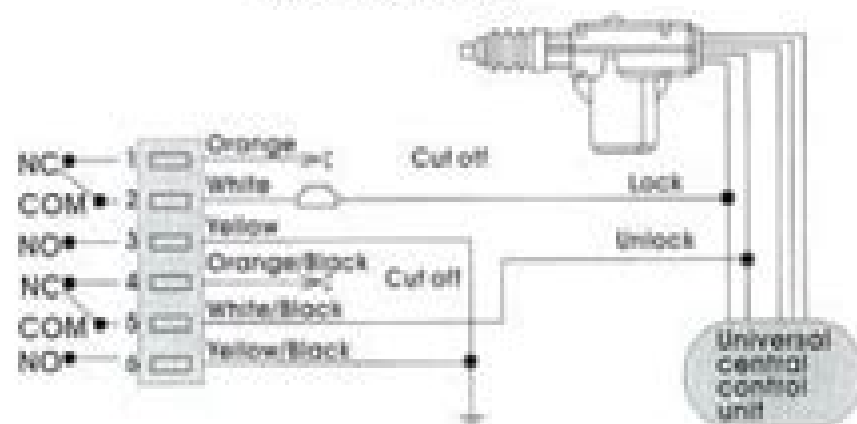
Negative trigger
