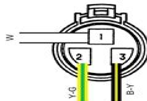
MA71 Alternator connector D
