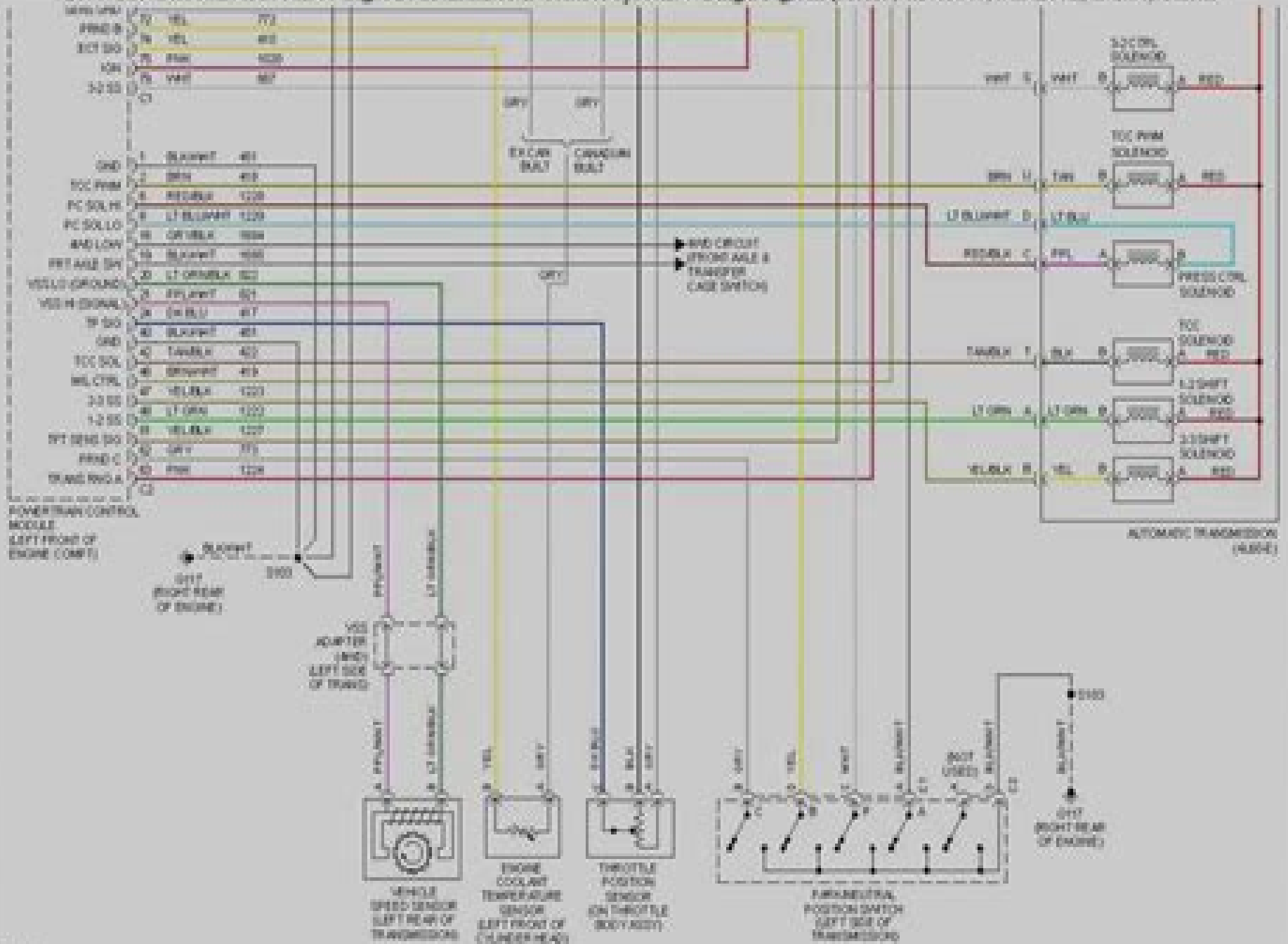
2000 Chevrolet Silverado 1500 Fig. 32: Transmission Control System Wiring Diagram (Sierra, Silverado, Suburban, Tahoe, Yukon)
