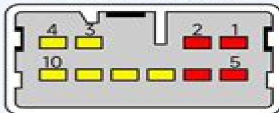
[ Connector A ]
