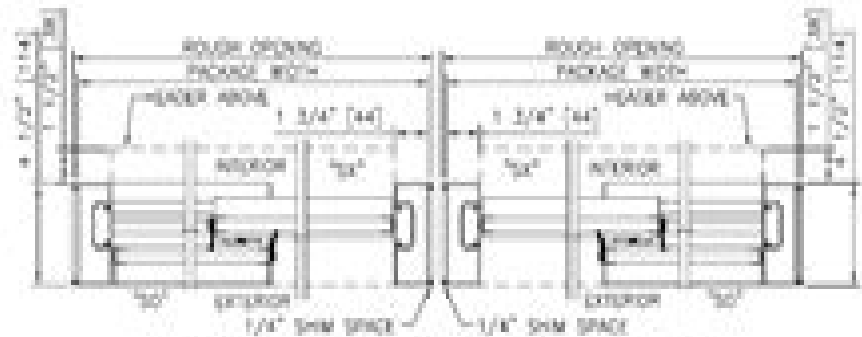
LEFT HAND HORIZONTAL SECTION RIGHT HAND ③ SCALE 1" = 1'-0"
